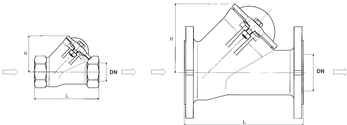
Rp 1 1/4 - 1 1/2 - 2 MODEL
